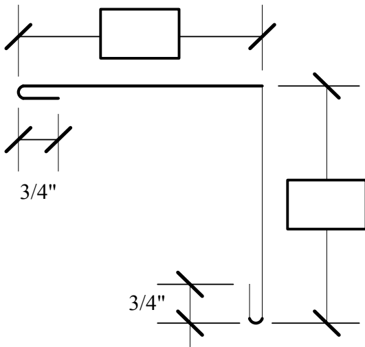
FLASHING "A"
