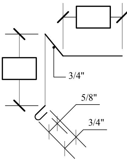
FLASHING "A"
